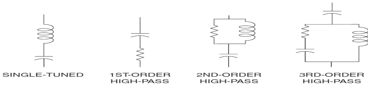
Figure 4.27 Common passive filter configurations.
