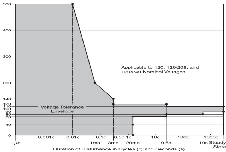
Fig 1.6 ITI curve for susceptibility of 120-V computer equipment.
