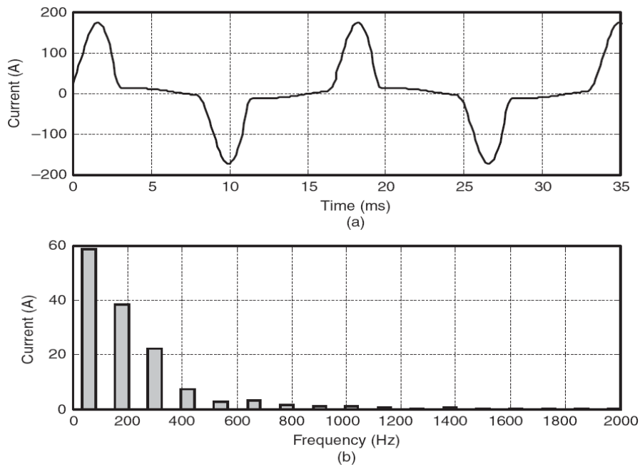
Figure 4.6 SMPS current and harmonic spectrum.
