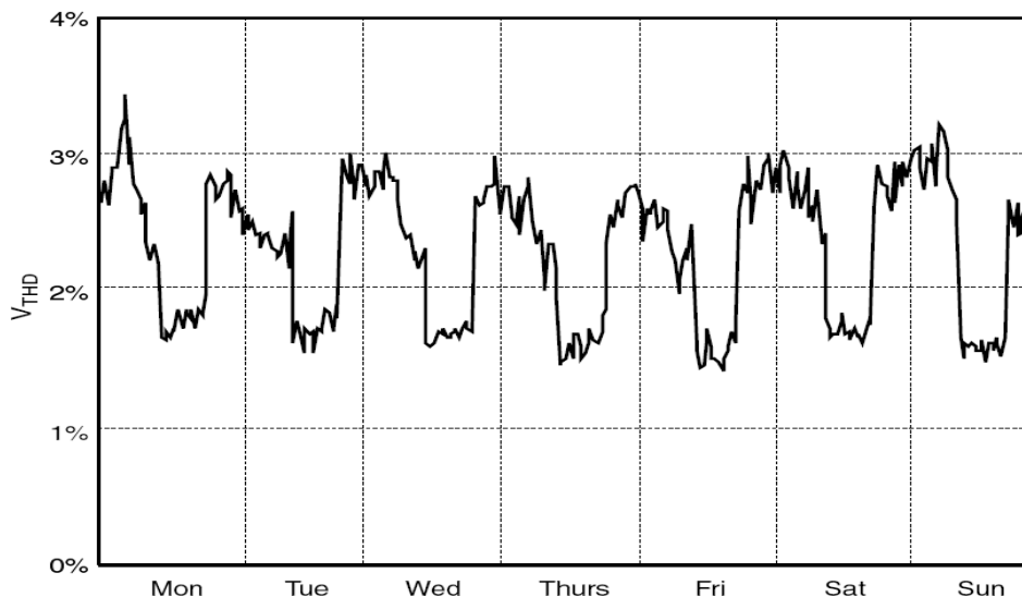
Fig 4.4 Variation of the voltage THD over a 1-week period.
