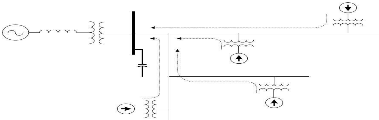
Figure 4.20 System with potential parallel resonance problems.
