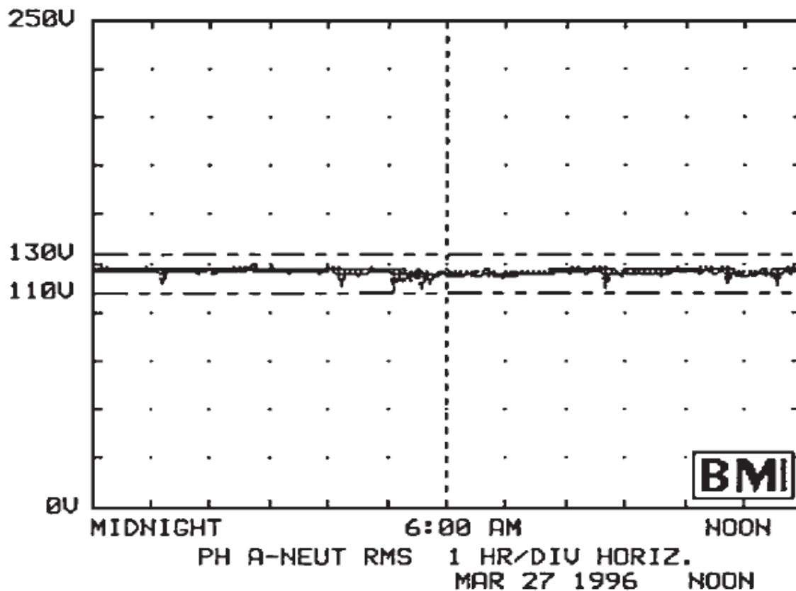
Figure 5.4 RMS voltage variations.
