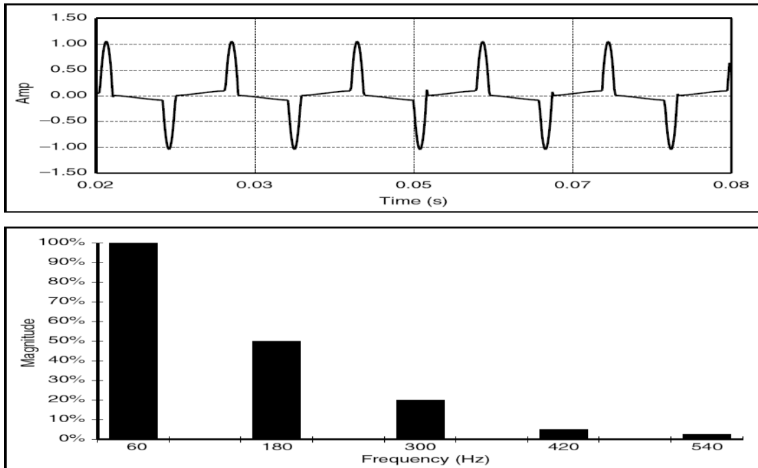
Figure 4.16 Transformer magnetizing current and harmonic spectrum.
