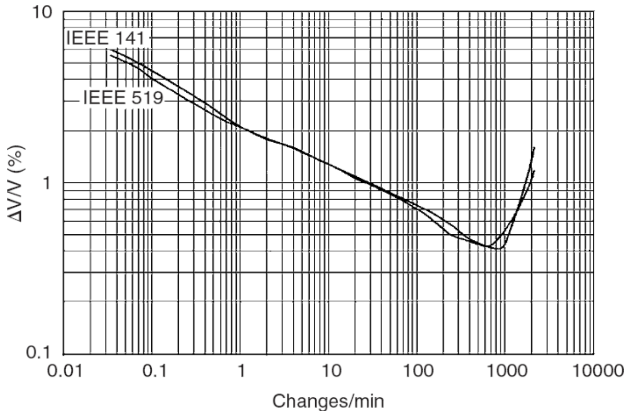
Figure 5.3 Flicker curves from IEEE Standards 141 and 519.
