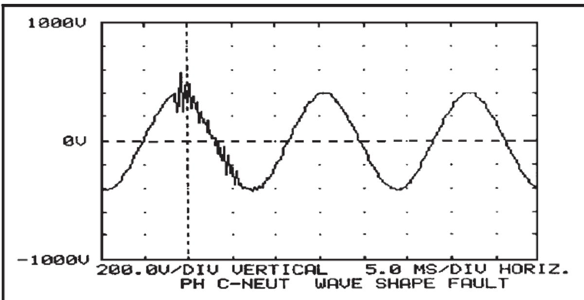
Figure 5.2 Graphics-based analyzer output.
