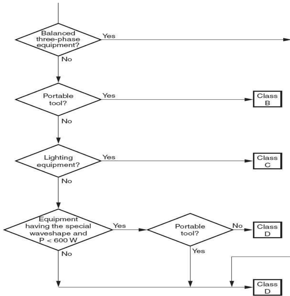
Figure 4.32 Flowchart for classifying equipment according to IEC 61000-3-2.
