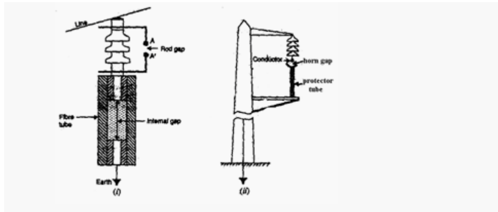
Typical expulsion arrester
