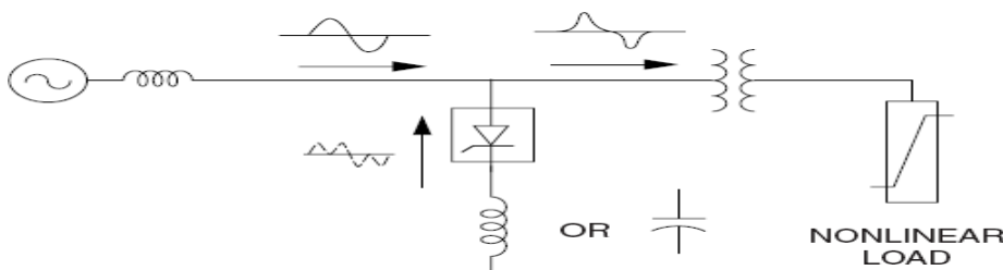
Figure 4.31 Application of an active filter at a load.
