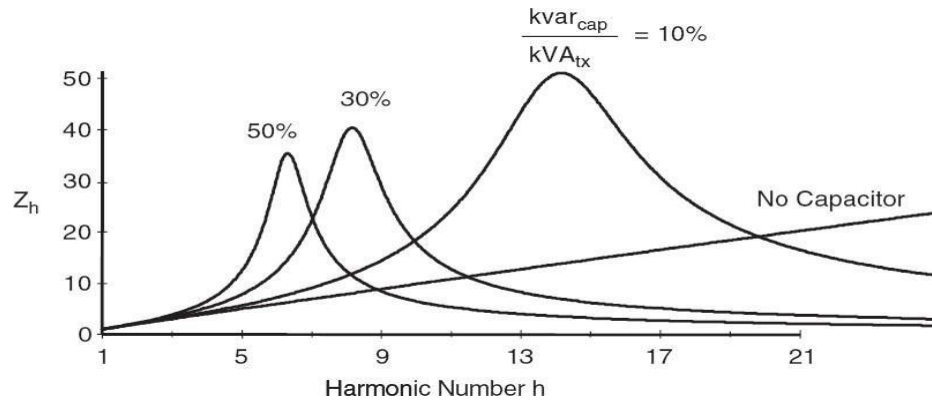
Fig 4.22 System frequency response as capacitor size is varied in relation to transformer.
