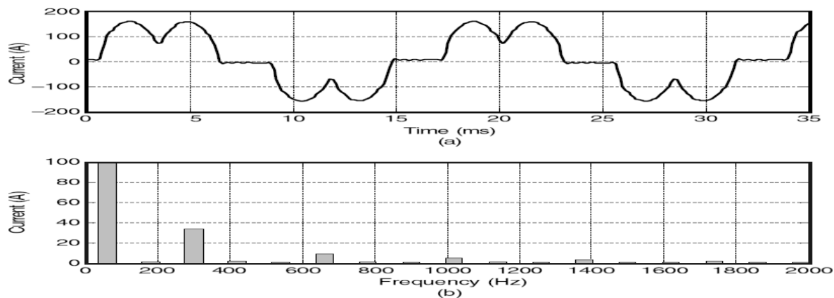
Figure 4.9 Current and harmonic spectrum for CSI-type ASD.
