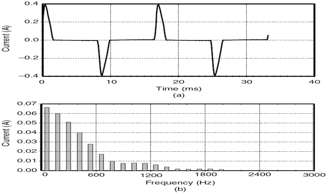
Figure 4.8 Fluorescent lamp with (a) electronic ballast current waveform and (b) its harmonic spectrum.
