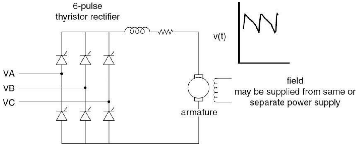
Figure 4.11 Six-pulse dc ASD.
