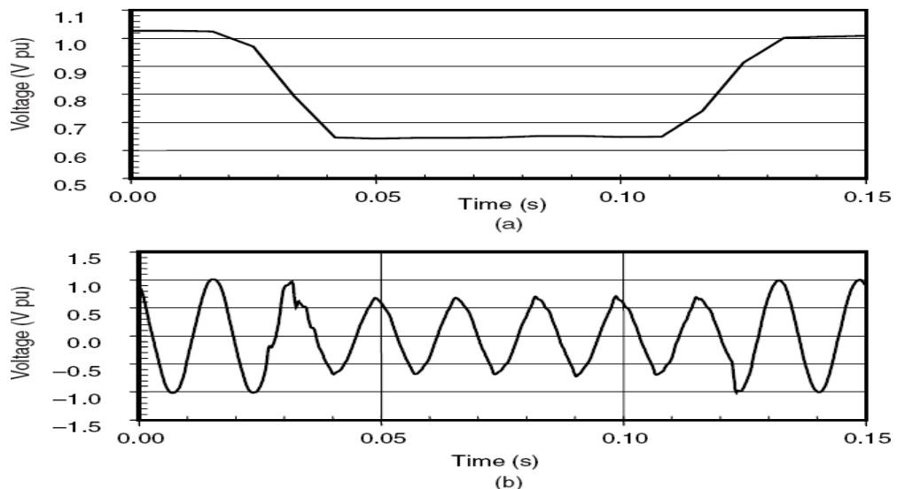
Figure 1.1 Voltage sag caused by an SLG fault. (a) RMS waveform for voltage sag event. (b) Voltage sag waveform.
