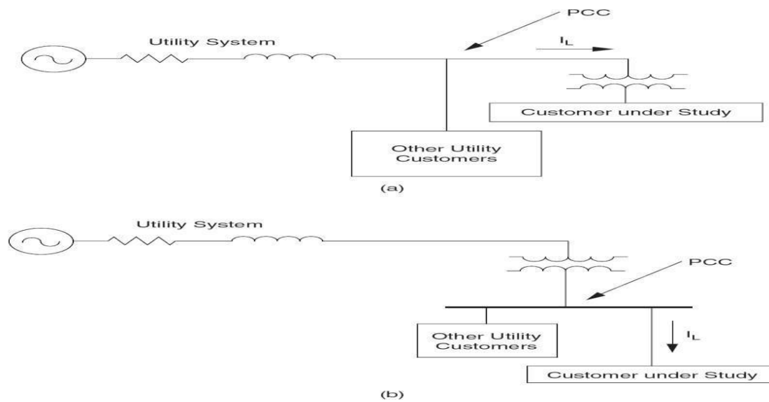
Figure 4.25 PCC selection depends on where multiple customers are served. (a) PCC at the transformer primary where multiple customers are served. (b) PCC at the transformer secondary where multiple customers are served.
