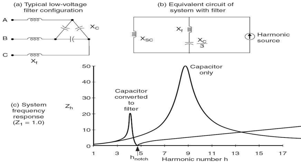
Figure 6.28 creating a fifth-harmonic notch filter and its effect on system response.
