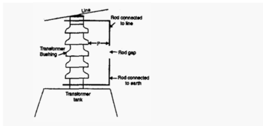
Typical rod gap arrester
