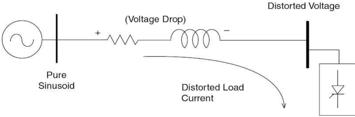
Fig 4.3 Harmonic currents flowing through the system impedance result in harmonic voltages at the load.
