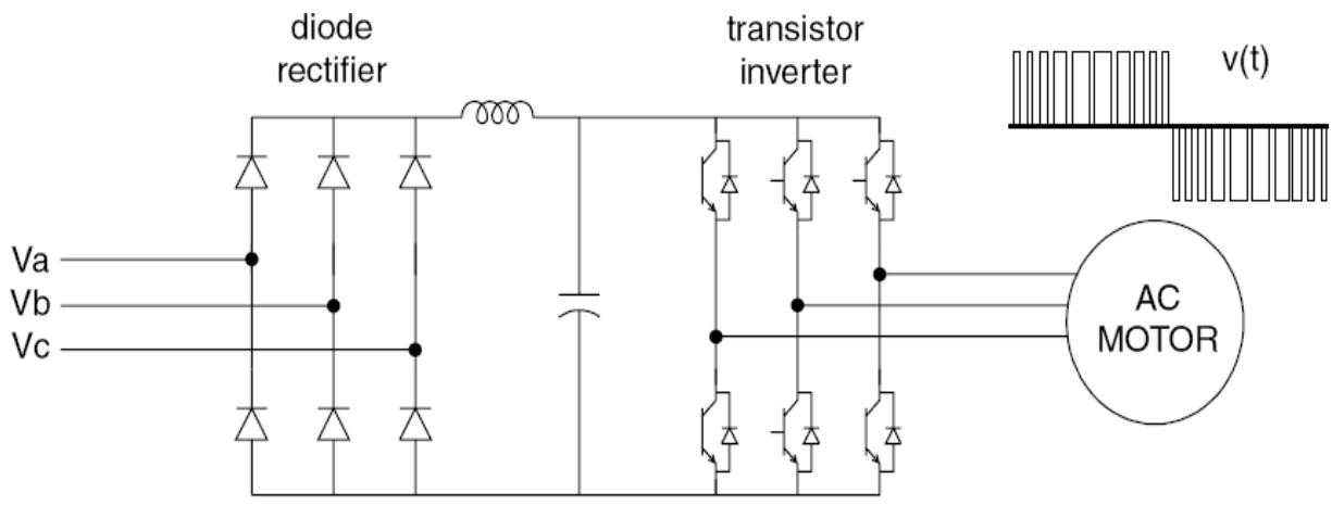
Figure 4.11 PWM ASD.
