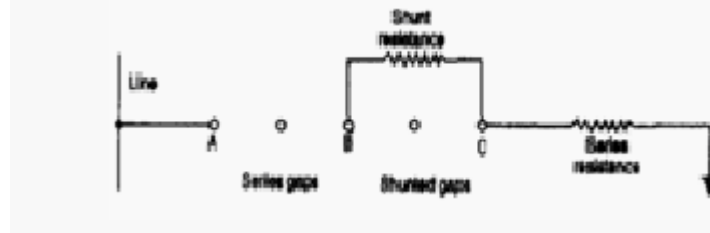
Typical multigap arrester
