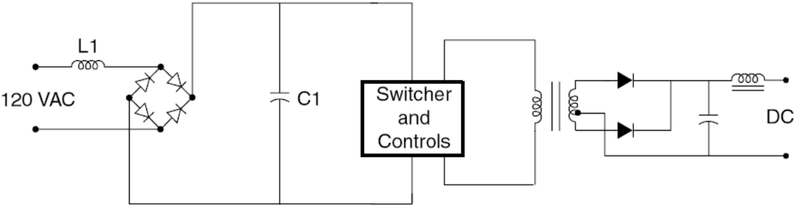
Figure 4.5 Switch-mode power supply.
