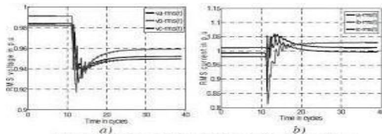
Figure 6. Voltage sag registered at node S90: a) rms voltage b) rms current.
